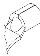
COLLETTO CHIUSO BRASATO DA LASTRA BARREL CLOSED BY SHEET WITH BRAZED FLAPS
